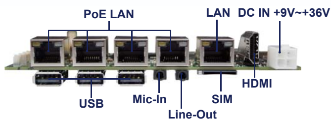
3I847NM Rear I/O
