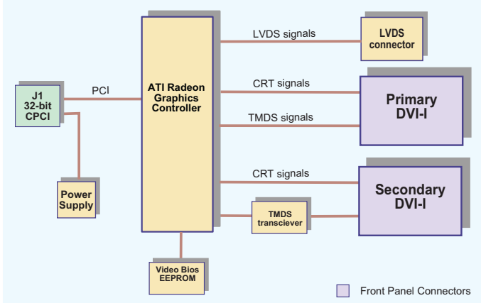
Block Diagramm CP332
